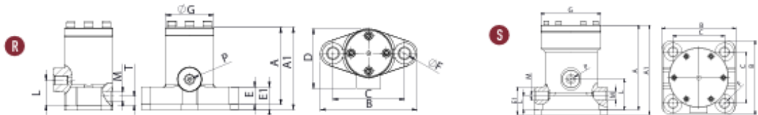
DIMENSIONAL SPECIFICATIONS
