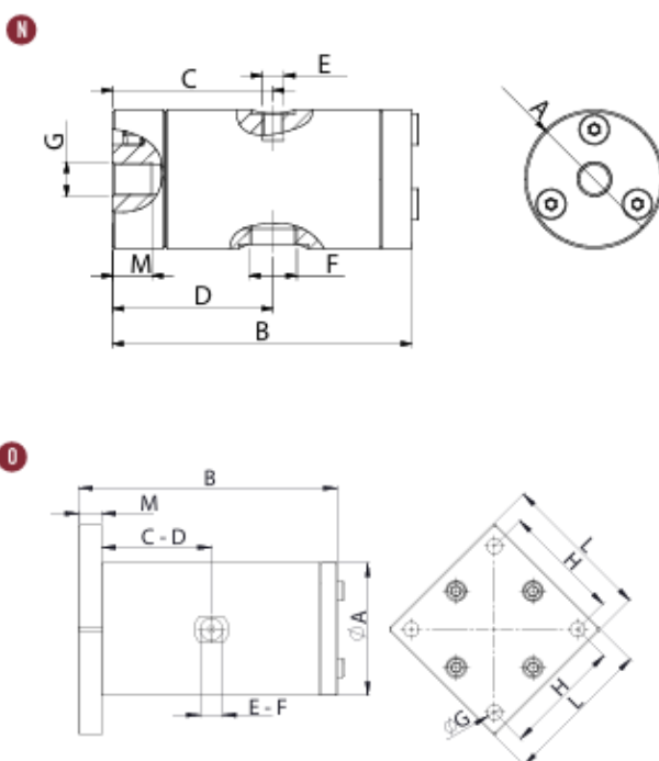
DIMENSIONAL SPECIFICATIONS
