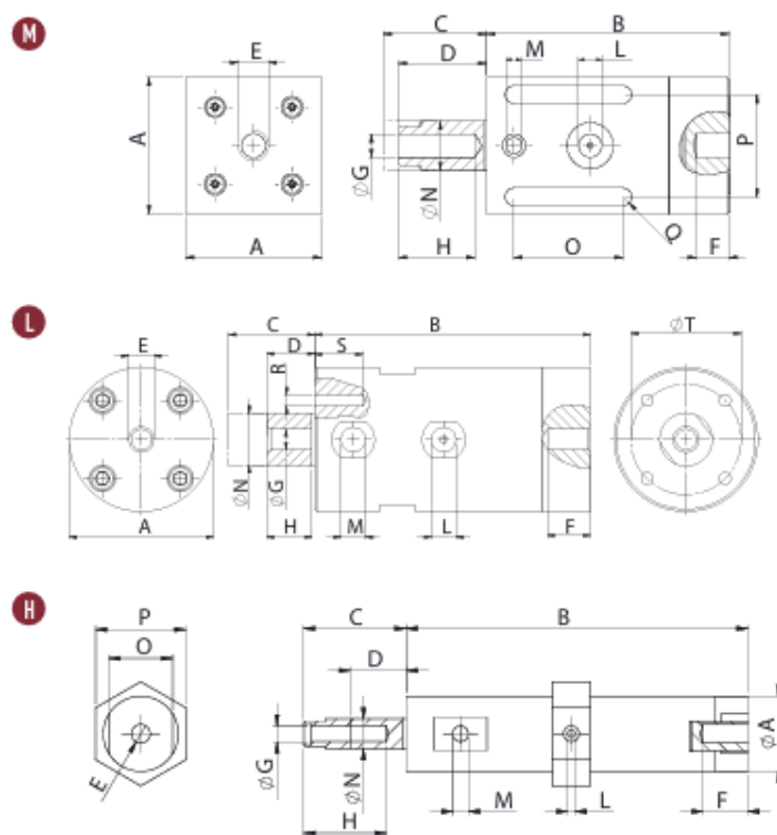
DIMENSIONAL SPECIFICATIONS
